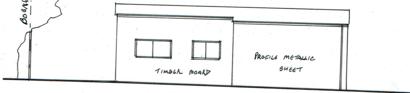
PROPOSED SOUTH EAST ELEVATION
